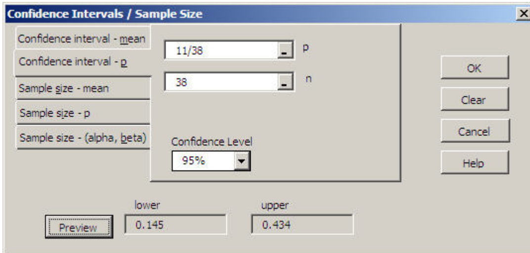
Figure 10. Proportion entered as a fraction.
