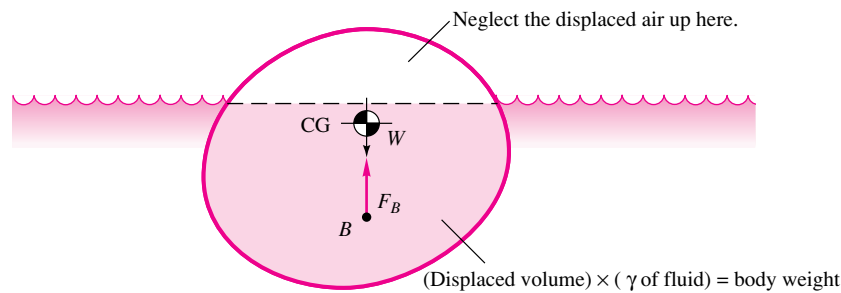
Fig. 2.17 Static equilibrium of a floating body.
