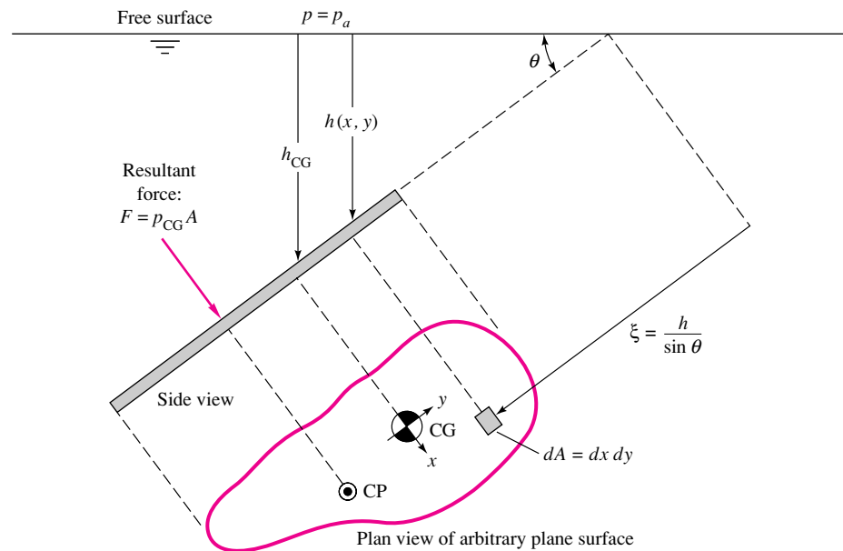
2.11 Hydrostatic force and center of pressure on an arbitrary plane surface of area A inclined at an angle \theta below the free surface.
