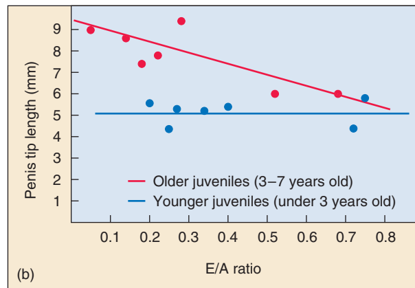
Alligator sexual development inhibited by contamination. (a) Ratio of estrogen/androgen (E/A) plasma concentrations in large juvenile alligators 3–7 years old. A relatively larger ratio in males (*) is atypical and indicates an estrogenic hormonal environment, as opposed to the expected androgenic hormonal environment. (b) Sexual development in male alligators, measured by penis length as a function of E/A ratio. In small juveniles under 3 years old, there is no apparent influence. In older juveniles 3–7 years old, there is a pronounced effect, higher E/A ratios retarding sexual development.
