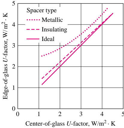
FIGURE 16-45 The edge-of-glass U -factor relative to the center-of glass U - for windows with various spacers.
