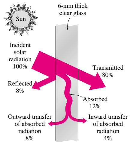
FIGURE 16-51 Distribution of solar radiation incident on a clear glass.
