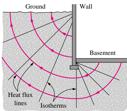
FIGURE 16-36 Radial isotherms and circular heat flow lines during heat flow from uninsulated basement.
