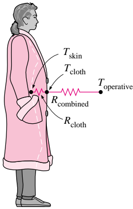
FIGURE 16-12 Simplified thermal resistance network for heat transfer from a clothed person.
