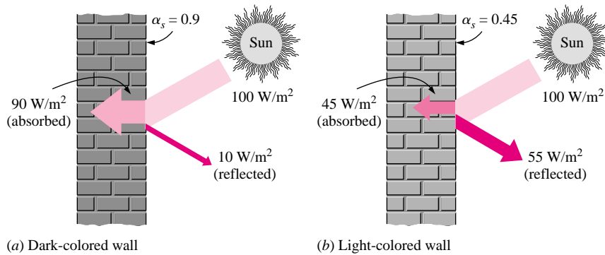
FIGURE 16-23 Dark-colored buildings absorb most of the incident solar radiation whereas light-colored ones reflect most of it.
