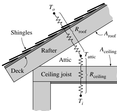
FIGURE 16-35 Thermal resistance network for a pitched roof-attic-ceiling combination for the case of an unvented attic.
