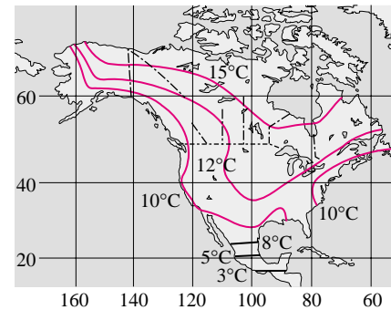
FIGURE 16-37 Lines of constant amplitude of annual soil temperature swings. (From ASHRAE Handbook of Fundamentals, Chap. 25, Fig. 6).
