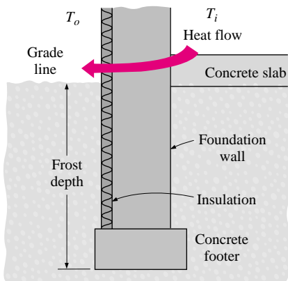
FIGURE 16–39 An on-grade concrete floor with insulated foundation wall.
