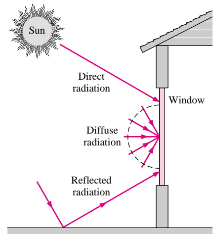
FIGURE 16-50 Direct, diffuse, and reflected components of solar radiation incident on a window.
