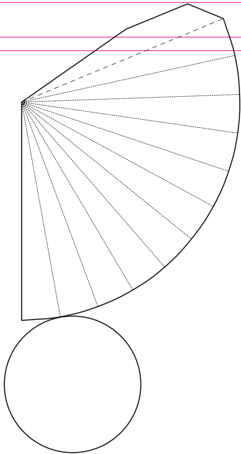
Pattern of a Cone to Be Made into Three-Dimensional Form
