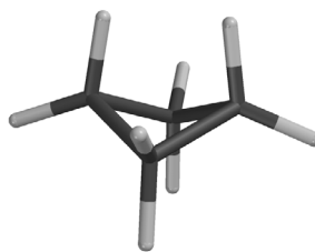
Cyclobutane
