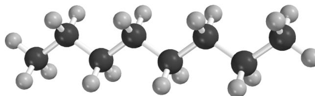
Octane
