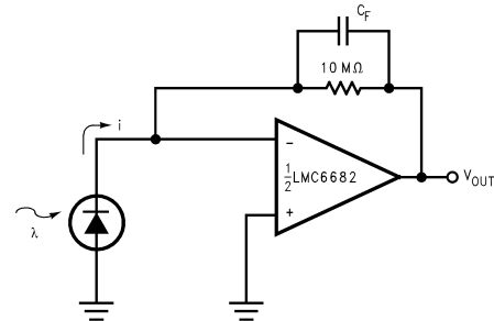
FIGURE 20. Photodiode Amplifier
