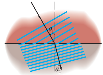
Figure 11.S1 Wave crests for a seismic wave incident on a boundary between two different kinds of rock. Not only does the wavelength (distance between wave crests) change at the boundary, the wave also refracts (changes its direction of propagation). The angles of incidence and refraction are \theta_1 and \theta_2 , respectively. The reflected wave is omitted for clarity.
